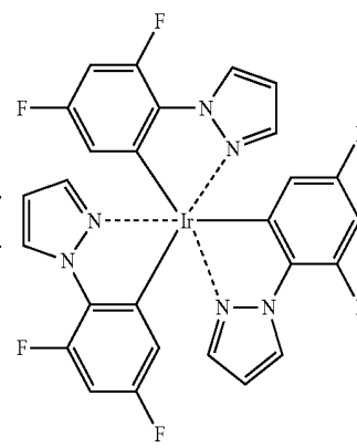
\text{Ir}(\text{dfppz})_3
