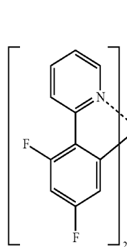
\text{F}_2\text{Irpic}
