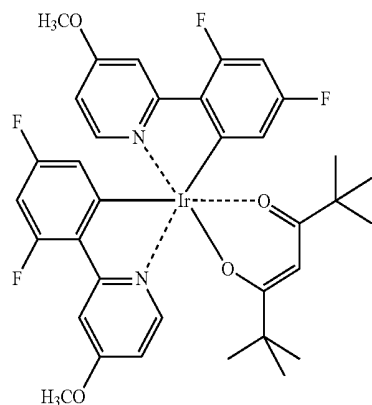
(\text{F}_2\text{ppy})_2\text{Ir}(\text{tmd})
