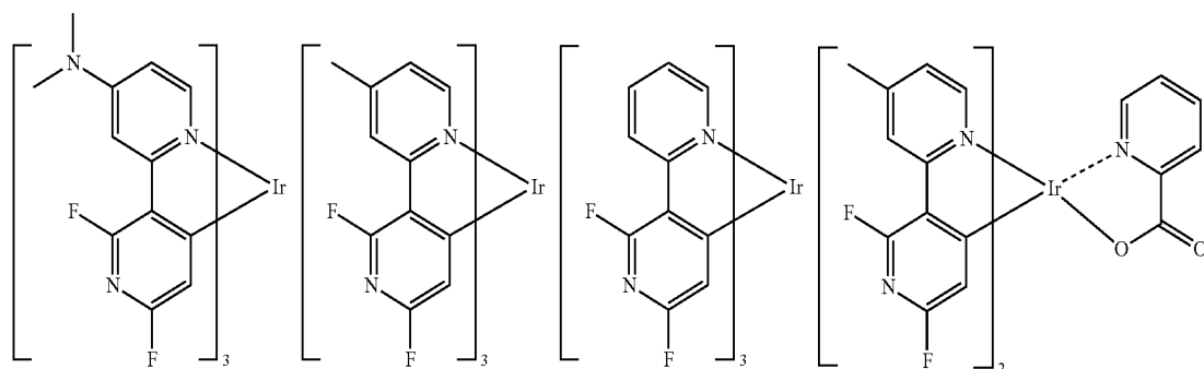
\text{F}_2\text{Irpic}
