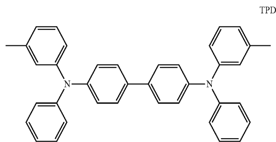
NPB
