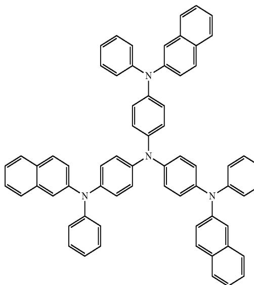
2-TNATA
